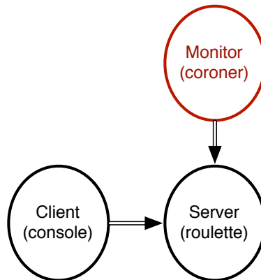
Figure 8—Adding monitoring
