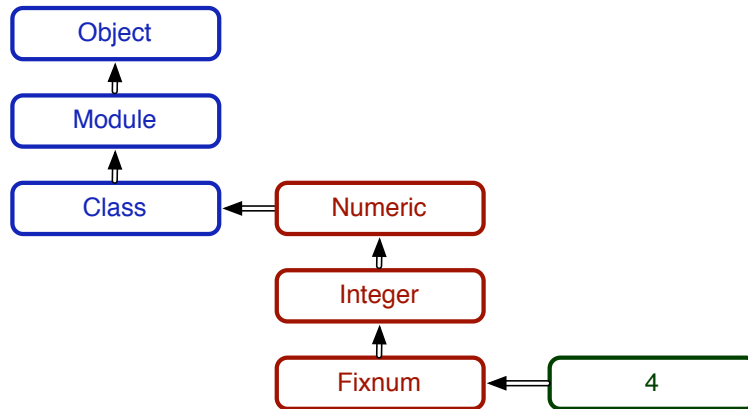
Figure 1—Ruby metamodel
